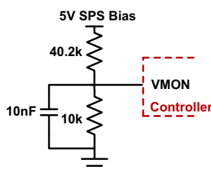
Figure 7. VMON Configuration
