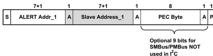
Figure 30. Alert Response Address (ARA, 0001_1001, 25h) for SMBus and PMBus, not used for I²C
