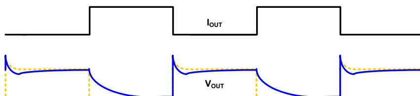
Figure 17. Load Transient Response when R-C Time Constant is Too Large
