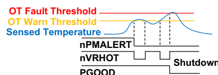
Figure 25. nVRHOT and Over-Temperature Shutdown
