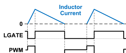
Figure 10. Diode Emulation PWM Signaling
