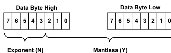
Figure 31. Linear 11 Data Format
