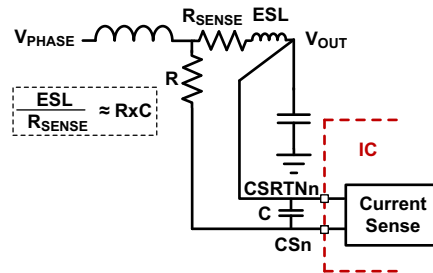
Figure 12. Sense Resistor in Series with Inductor
