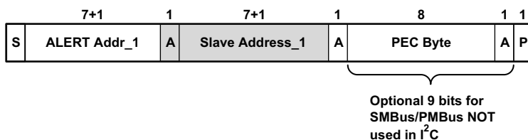
Figure 29. Alert Response Address (ARA, 0001_1001, 25h) for SMBus and PMBus, not used for I 2 C
