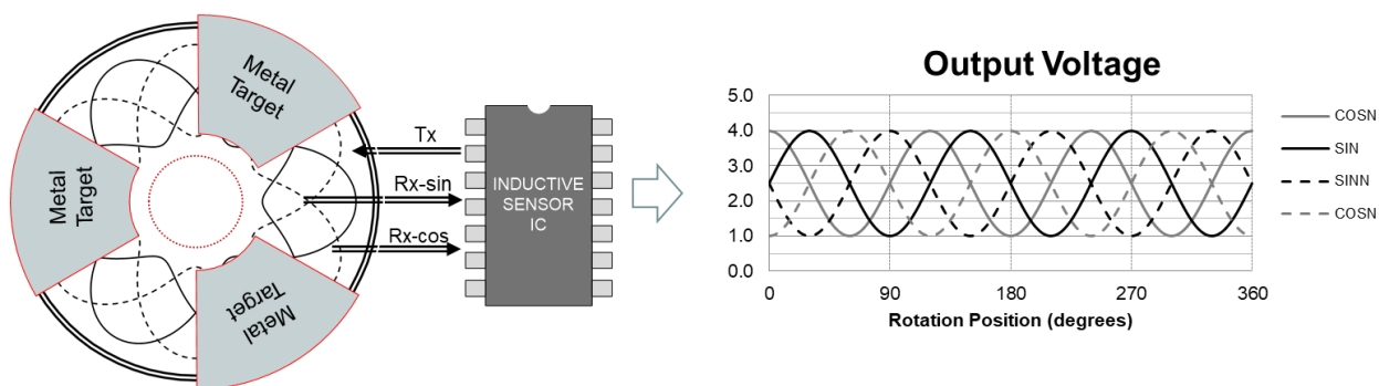
Figure 25. Coil Design and Signal Output for a 3 \times 120^\circ Rotary Sensor
