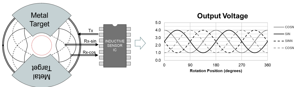
Figure 24. Coil Design and Signal Output for a 2 \times 180^\circ Rotary Sensor
