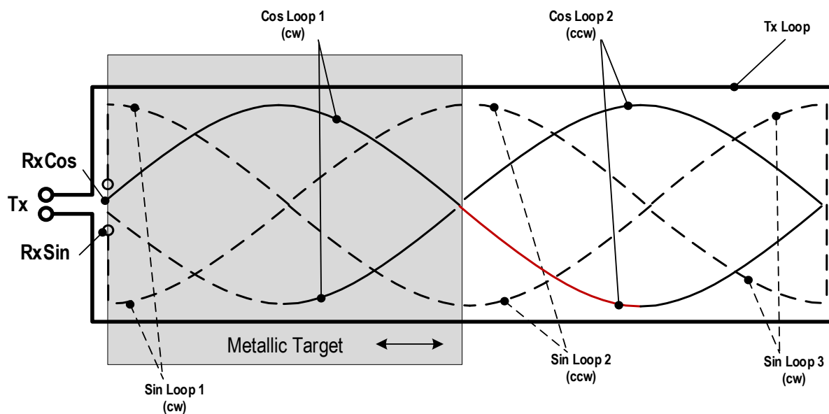
Figure 6. Coil Design for a Linear Motion Sensor
