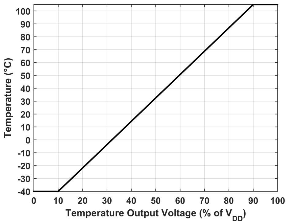
Figure 9. Temperature vs. VT Output Analog Voltage
