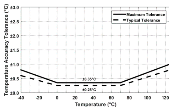
Figure 6. HS4013 Temperature Sensor Accuracy Tolerance
