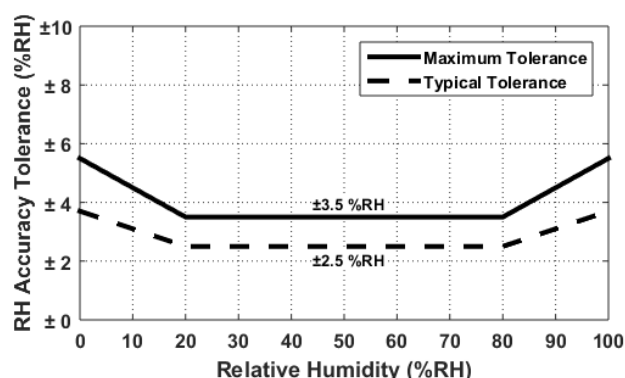
Figure 3. HS4013 RH Accuracy Tolerance at 25°C
