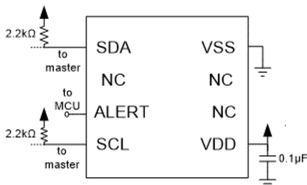
Figure 24. HS400x Application Circuit (Top View)
