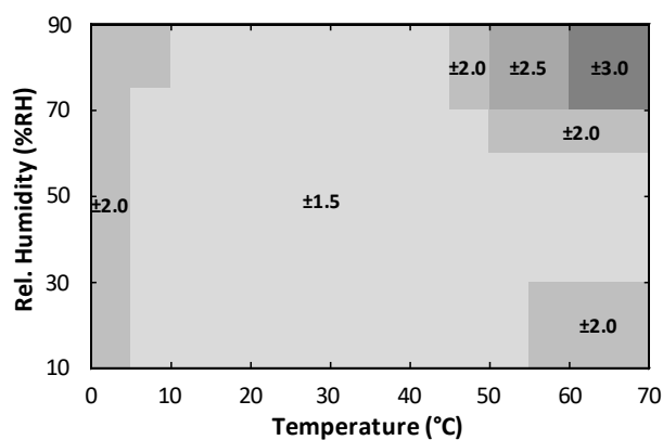
Figure 2. HS4001 RH Accuracy over Temperature
