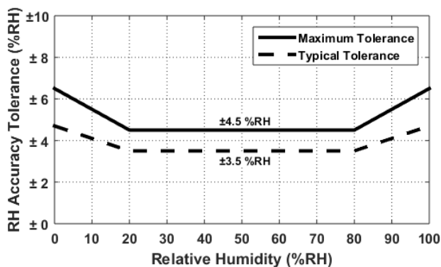
Figure 7. HS4004 RH Accuracy Tolerance at 25°C
