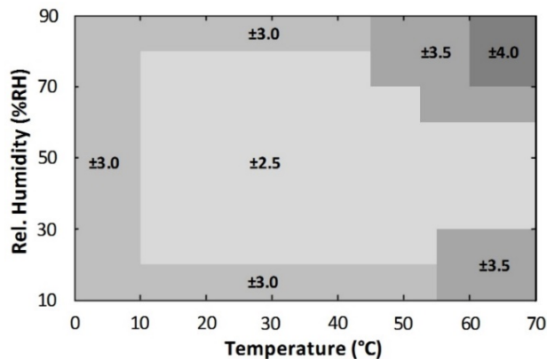
Figure 6. HS4003 RH Accuracy over Temperature
