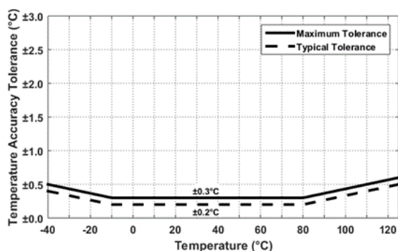
Figure 9. HS4001/HS4002 Temperature Sensor Accuracy Tolerance
