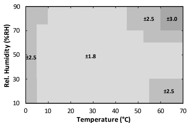
Figure 4. HS4002 RH Accuracy over Temperature
