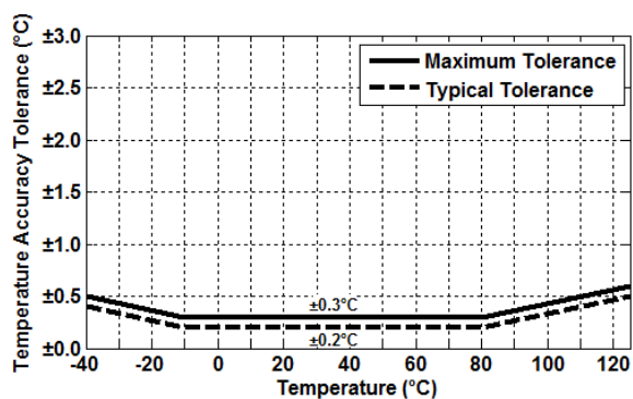
Figure 8. HS3101/HS3102 Temperature Sensor Accuracy Tolerance
