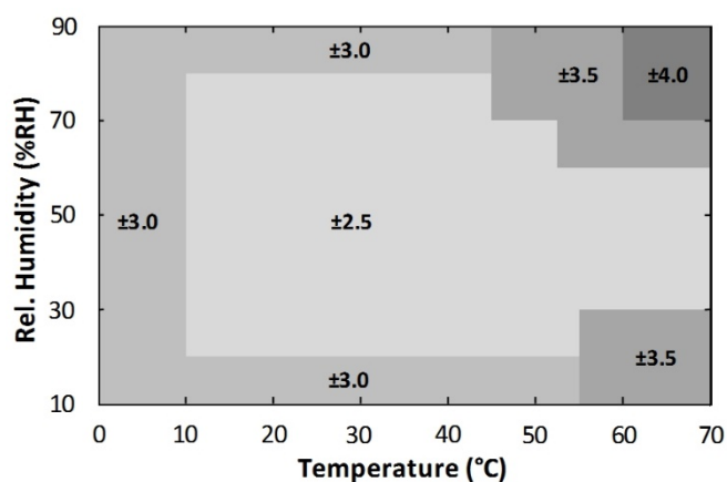
Figure 7. HS3103 RH Accuracy over Temperature
