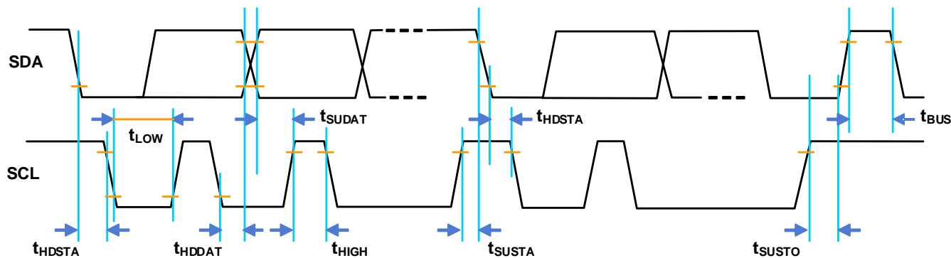
Figure 10. Timing Diagram
