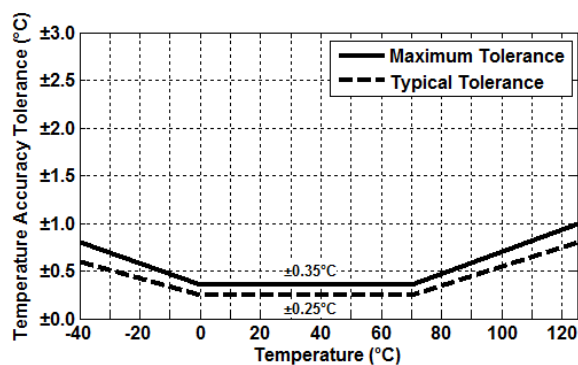
Figure 9. HS3103 Temperature Sensor Accuracy Tolerance
