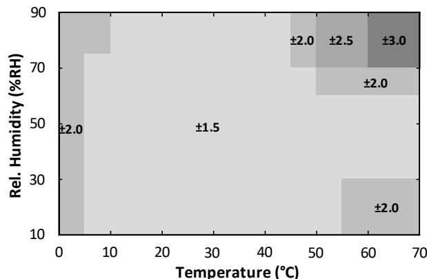
Figure 3. HS3101 RH Accuracy over Temperature
