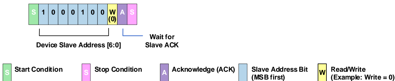
Figure 12. Measurement Request
