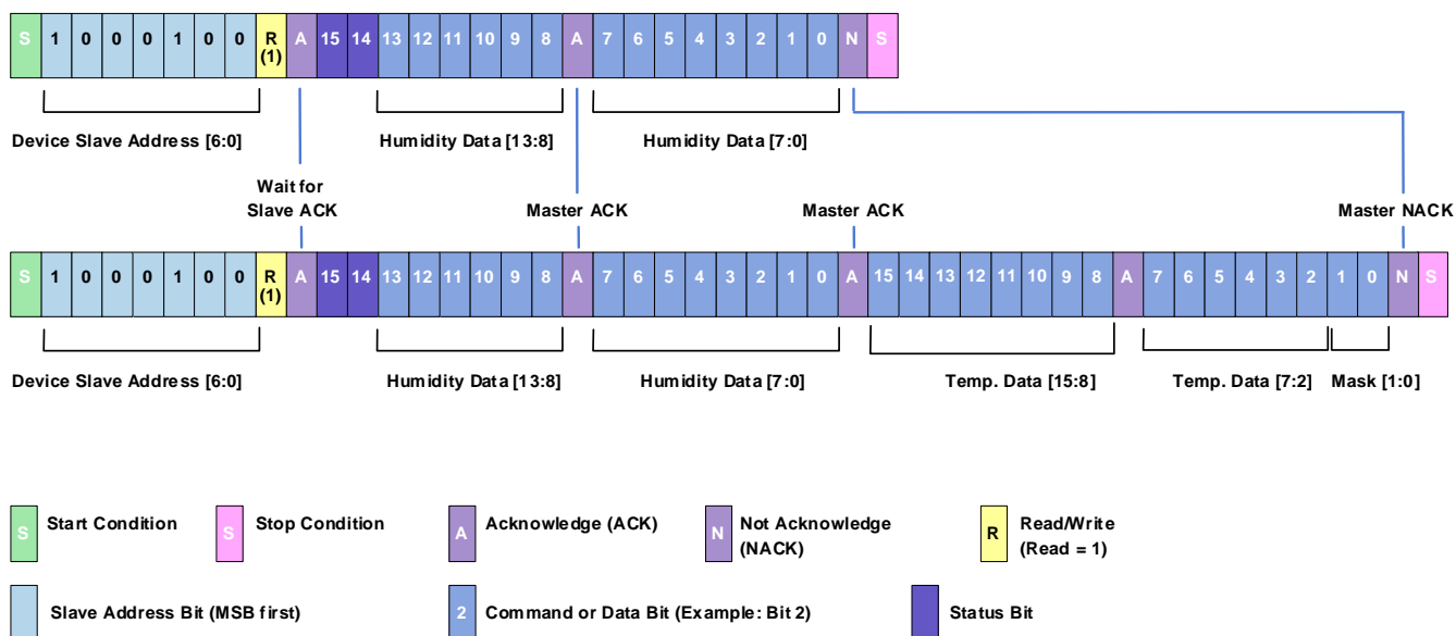
Figure 12. Data Fetch
