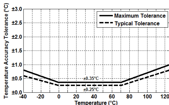
Figure 8. HS3003 Temperature Sensor Accuracy Tolerance
