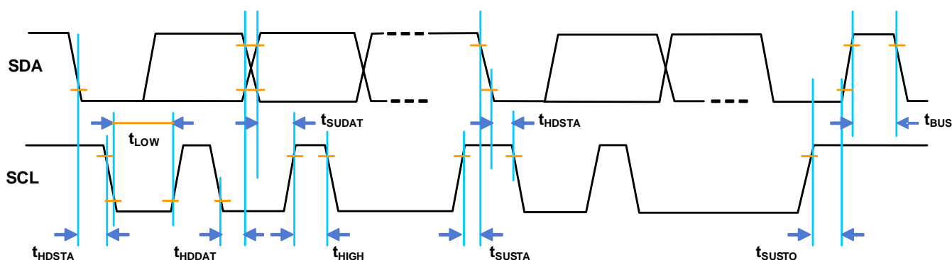
Figure 9. Timing Diagram
