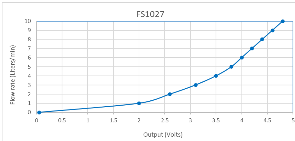
Figure 1. Analog Output Curve
