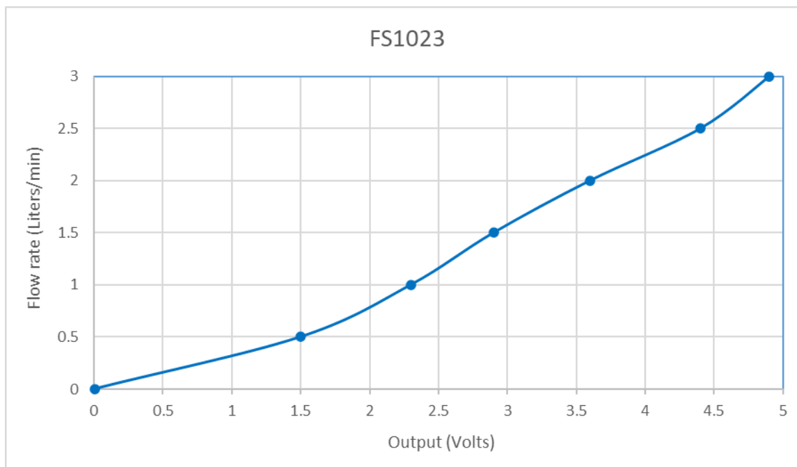
Figure 1. Analog Output Curve
