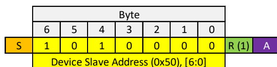
Figure 7. Flow Data Read Command
