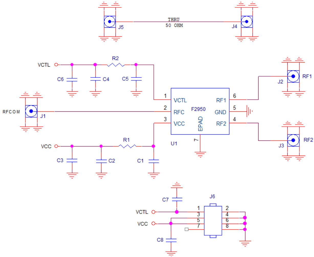
Figure 20. Electrical Schematic
