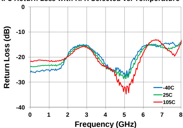
RFC Return Loss with RFX Selected vs. Temperature
