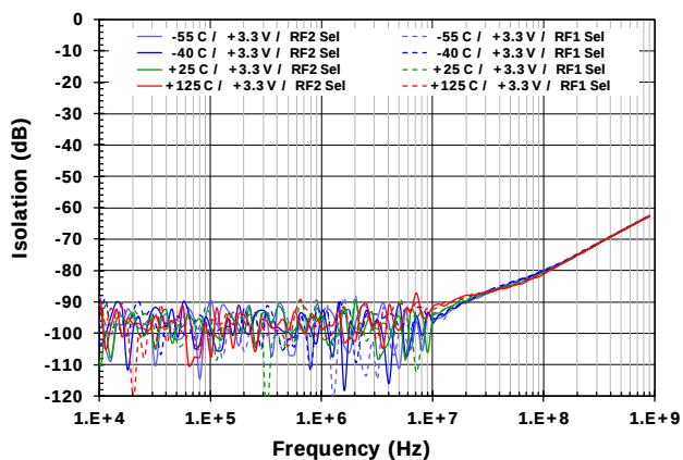
Figure 6. Isolation vs. Temperature [RFC → RF1 / RF2]
