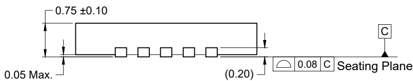
SIDE VIEW
