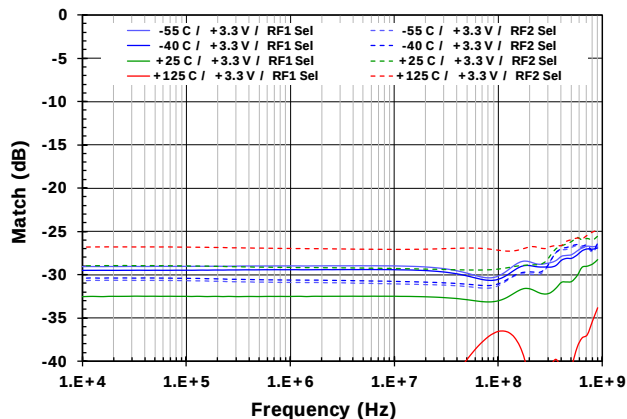
Figure 18. RF2 Return Loss vs. Temperature
