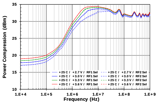
Figure 28. Input Power Compression vs. Voltage
