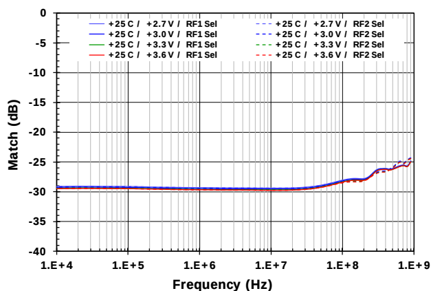
Figure 24. RFC Return Loss vs. Voltage
