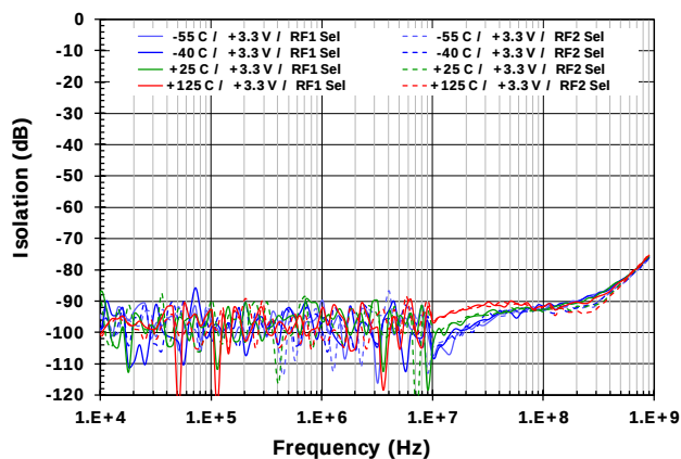
Figure 10. Isolation vs. Temperature [RF1 → RF2]
