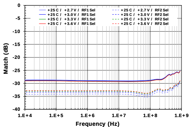
Figure 16. RF1 Return Loss vs. Voltage
