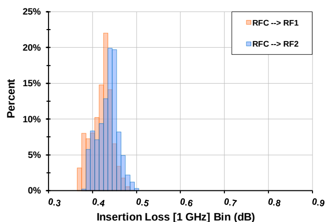
Figure 38. Insertion Loss [RF = 1GHz]
