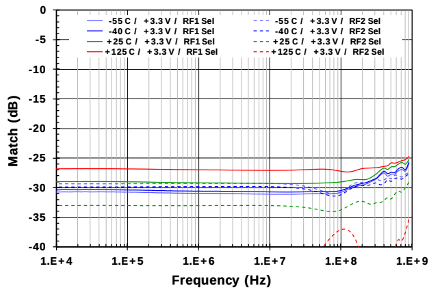
Figure 14. RF1 Return Loss vs. Temperature
