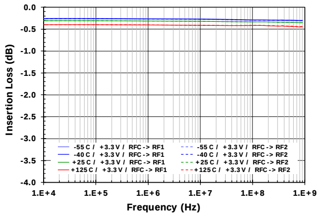
Figure 2. Insertion Loss vs. Temperature
