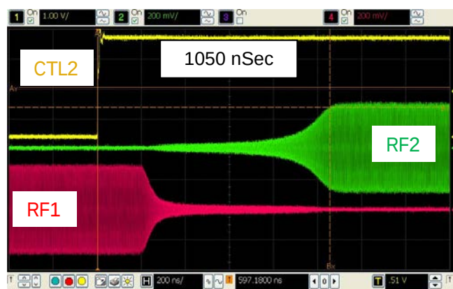
Figure 37. Switching Time [ T_{AMB} = -40^{\circ}\text{C} , 3.3V]
