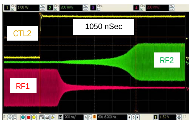
Figure 36. Switching Time [ T_{AMB} = 25^{\circ}\text{C} , 3.3V]
