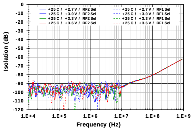
Figure 8. Isolation vs. Voltage [RFC → RF1 / RF2]
