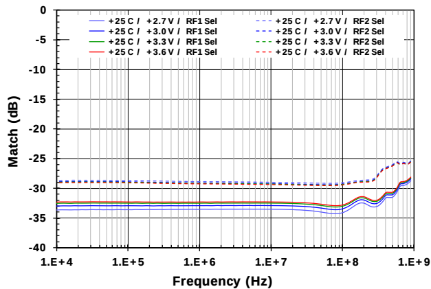
Figure 20. RF2 Return Loss vs. Voltage
