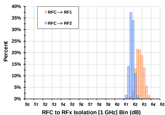
Figure 41. Isolation [RF = 1GHz]
