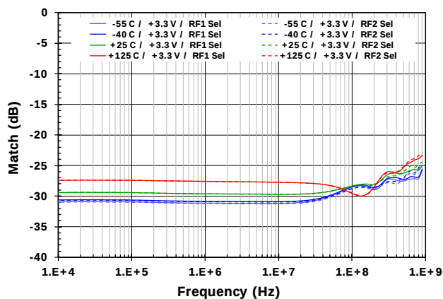
Figure 22. RFC Return Loss vs. Temperature
