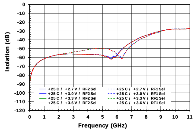
Figure 9. Isolation vs. Voltage [RFC → RF1 / RF2]
