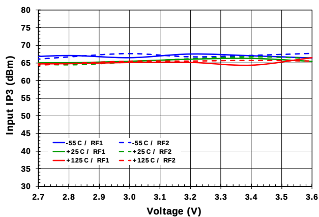
Figure 32. Input IP3 [ 2GHz]
