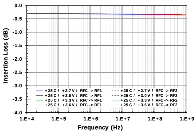
Figure 4. Insertion Loss vs. Voltage
