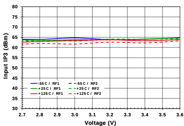
Figure 34. Input IP3 [ 4GHz]
