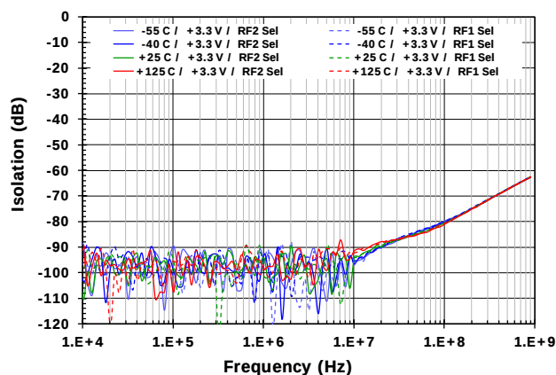
Figure 12. Isolation vs. Voltage [RF1 → RF2]
