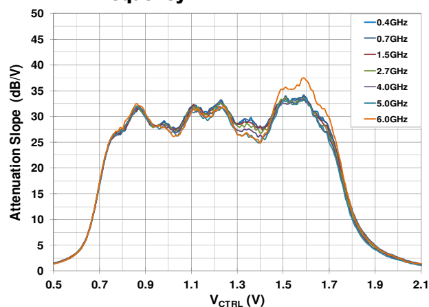
Figure 9. Attenuation Slope vs. V_{CTRL} over Frequency
