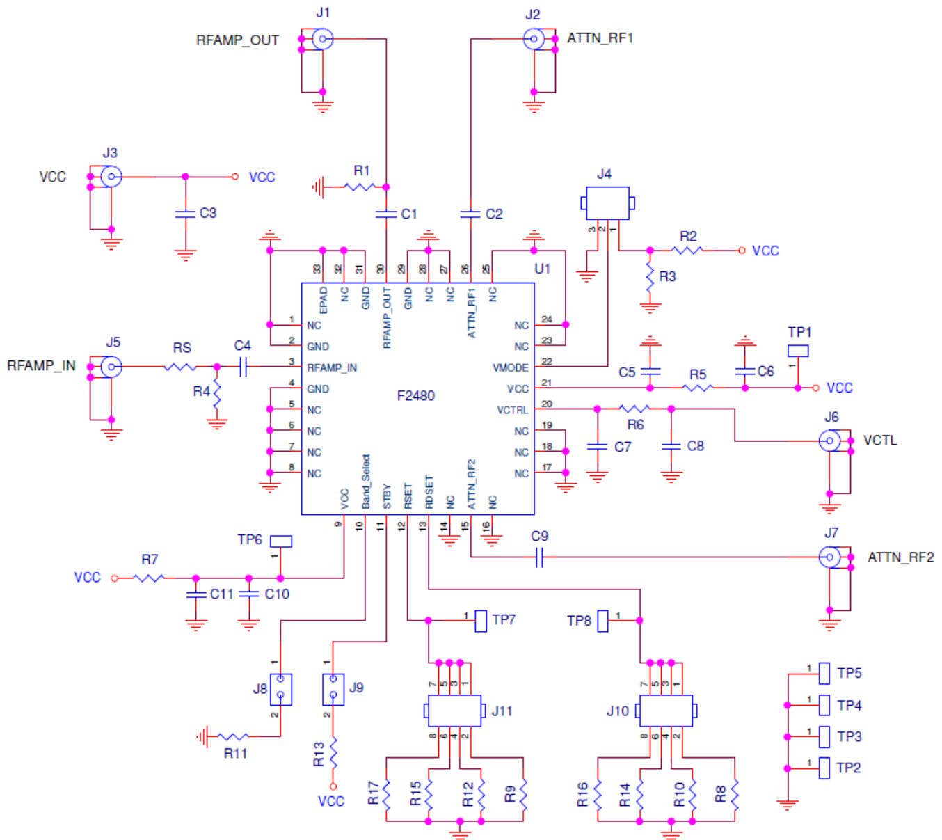
Figure 86. Electrical Schematic
