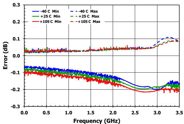
Figure 14. Worst-Case Step Accuracy
