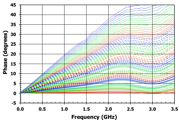
Figure 12. Worst-Case Absolute Accuracy Error
