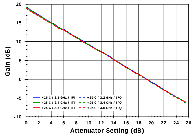
Figure 92. Gain vs. Attenuator Setting [High Side LO, RF Y , at RF Frequency]
