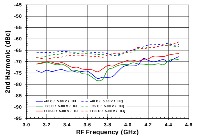
Figure 56. 2nd Harmonic vs. T_{case} [High Side LO, RF_Y , P_{IF} = -6 dBm]
