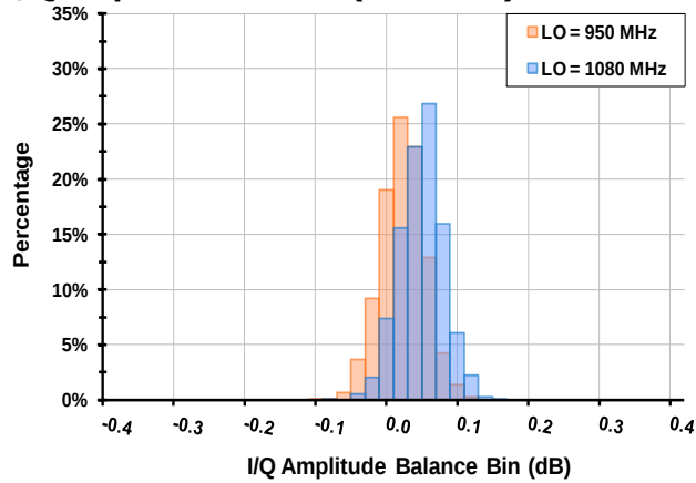
I/Q Amplitude Balance (N = 2724)
