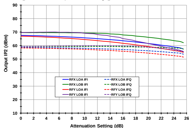
OIP2 [0.8 GHz RF, HiSide Inj.]
