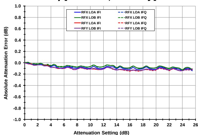
ATTN Accuracy [0.8 GHz RF, HiSide Inj.]
