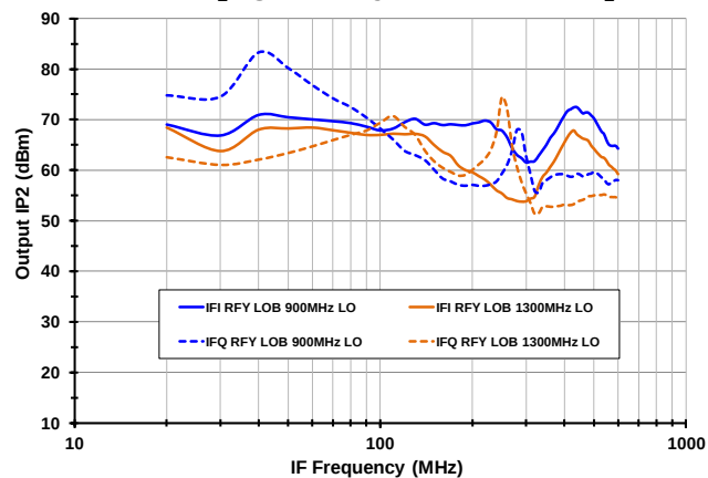
OIP2 Flatness [High Side Injection, RF_Y LO_B]
