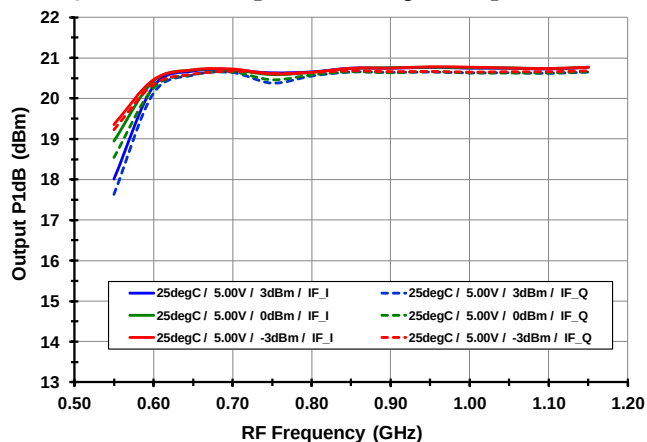
P1dB 0 vs. LO level [Low Side Injection]
