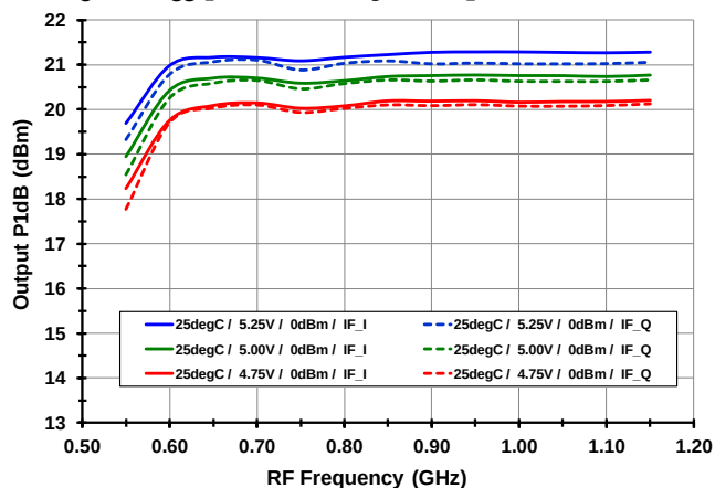
P1dB 0 vs. V CC [Low Side Injection]
