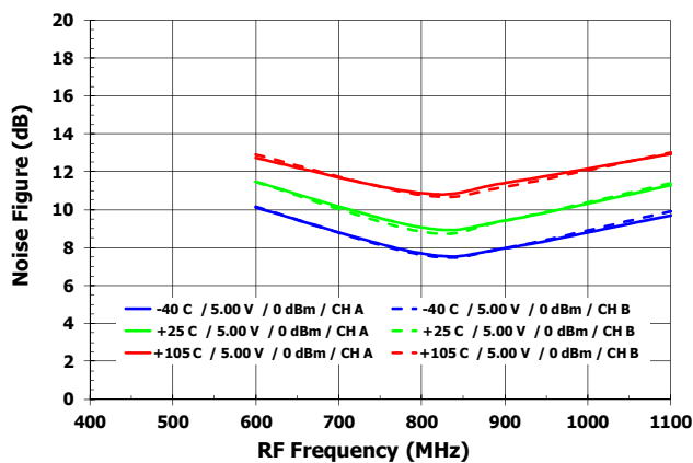
Noise Figure with Blocker [ NF_{MIXR\_BLK} ]
