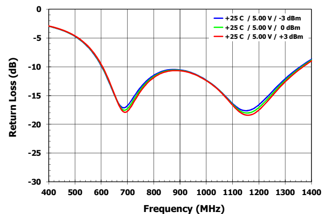
Mixer IF Output Return Loss [ S_{22_{MIXR\_IF}} ]
