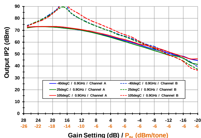
Output IP2 [RF=0.9 GHz]
