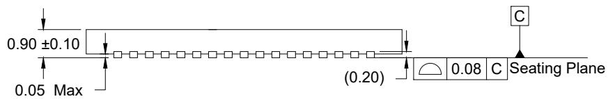
SIDE VIEW
