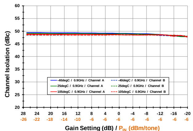
Channel Isolation [RF=0.9 GHz]
