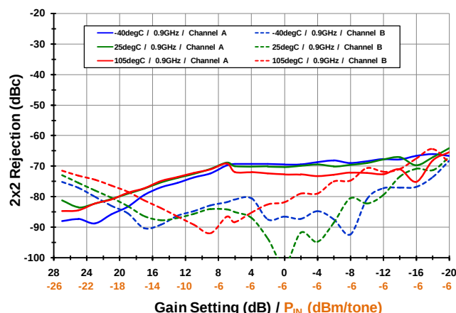
2LO-2RF Rejection [RF=0.9 GHz]
