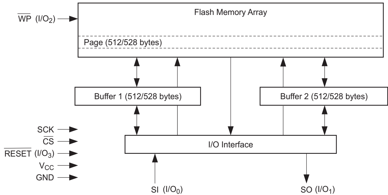
Figure 2-1. Block Diagram
