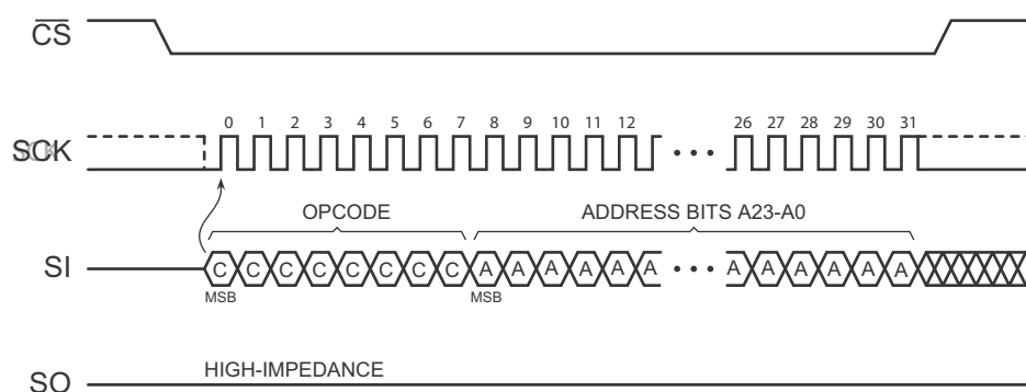
Figure 20. Block Erase
