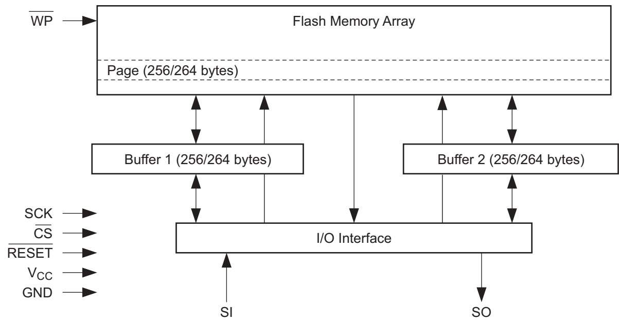
Figure 2-1. Block Diagram
