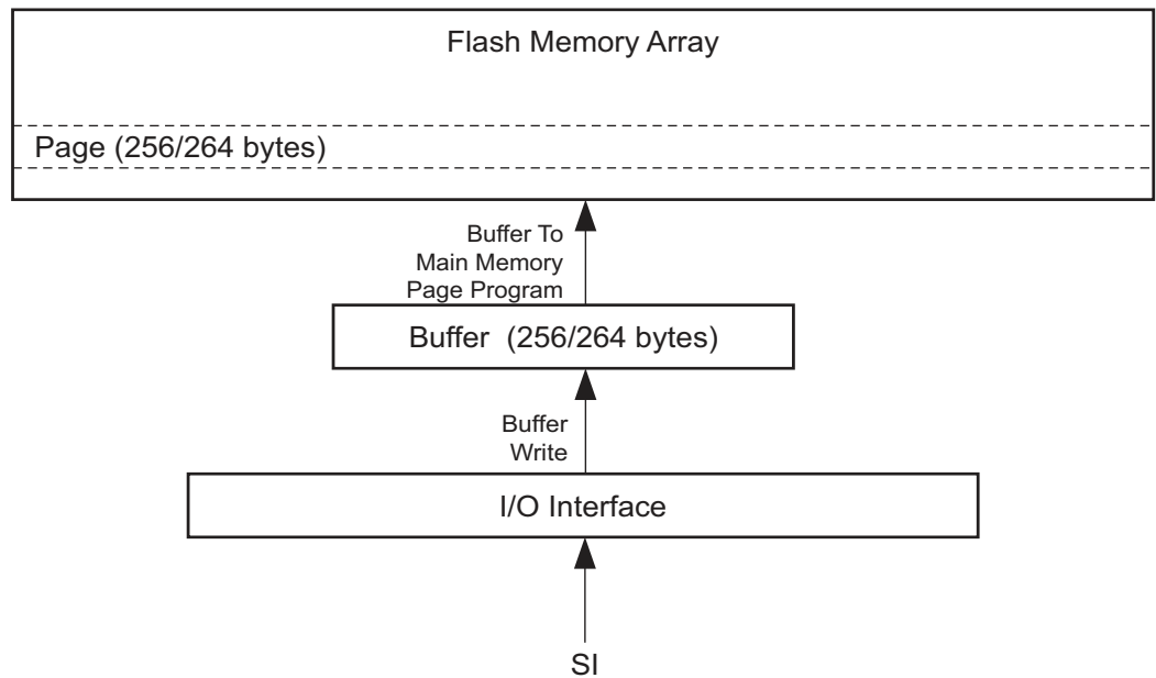
Figure 23-1. Block Diagram
