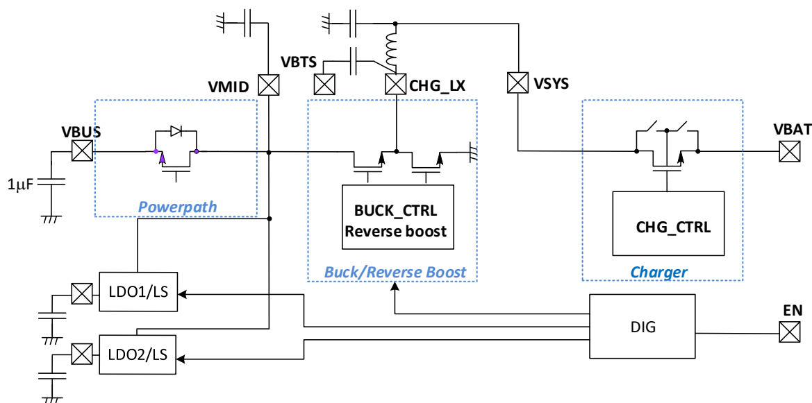
Figure 14: EN Pin Example
