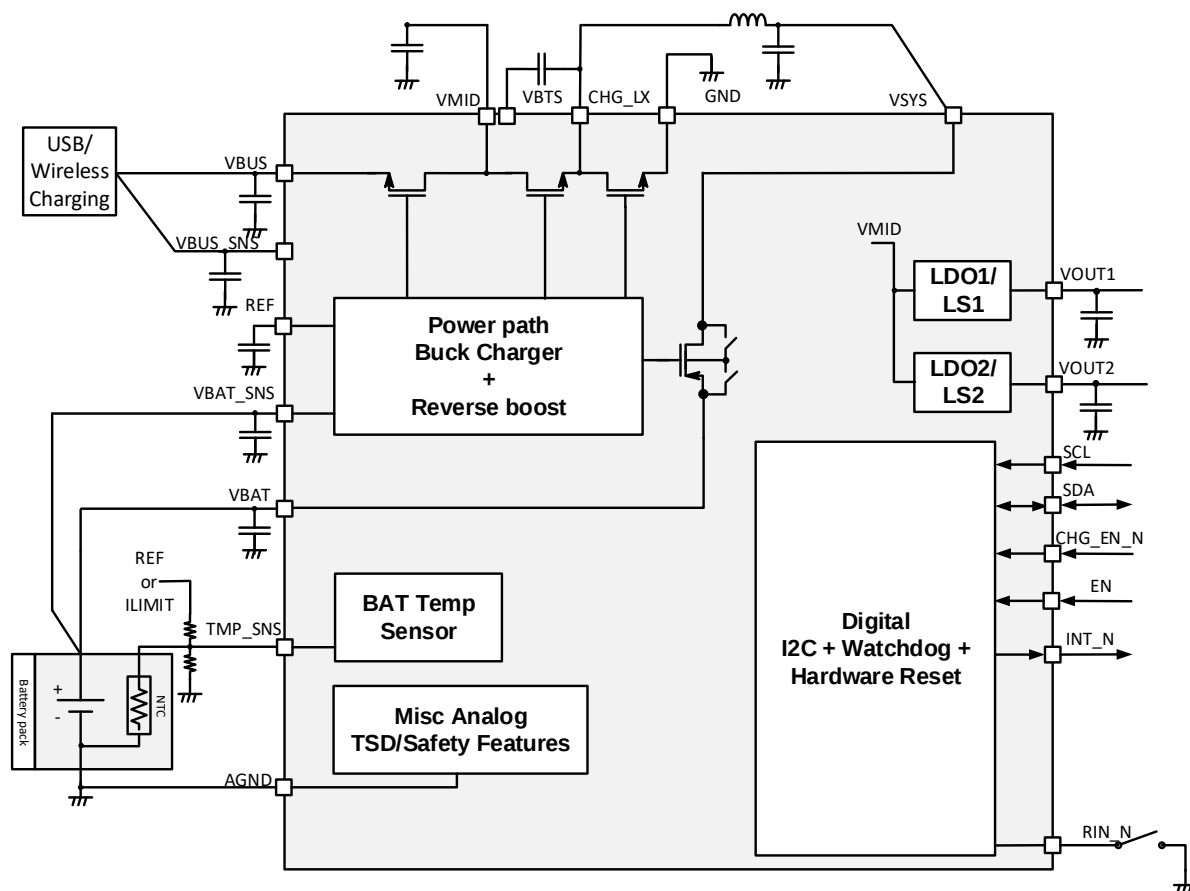
Figure 1: System Diagram
