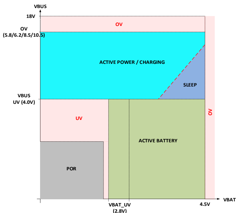
Figure 3: Regions of Operation
