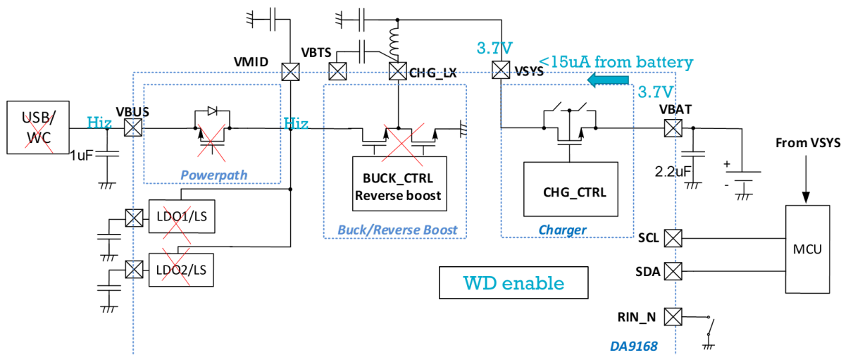
Figure 5: Standby Mode
