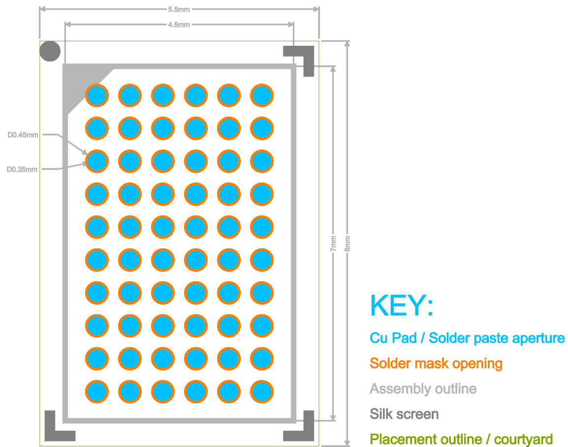
Figure 13: DA9141 Footprint
