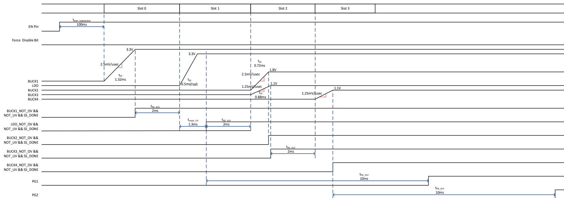
Figure 7: Timing Diagram Example for Power-Up
