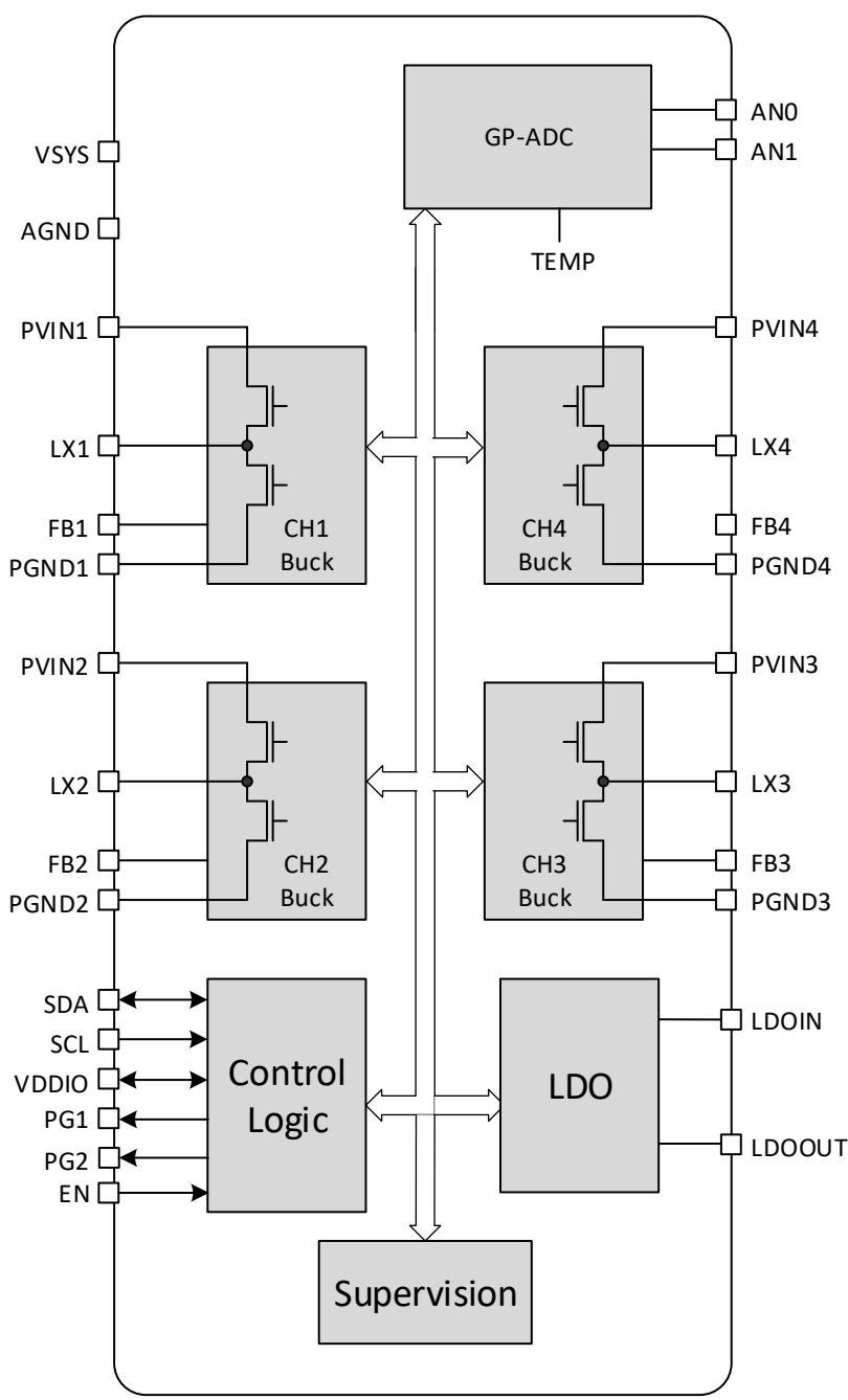
Figure 2: Block Diagram
