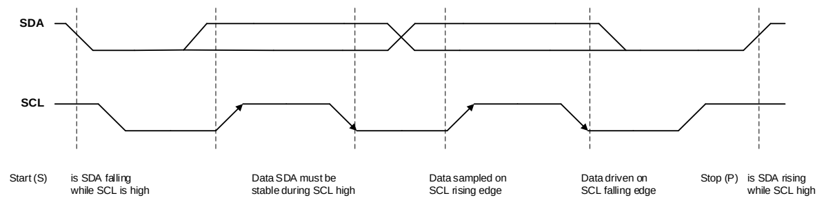
Figure 11: I 2 C Start (S) and Stop (P)
