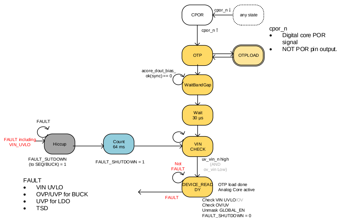
Figure 6: FSM States
