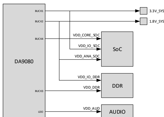
Figure 1: System Diagram
