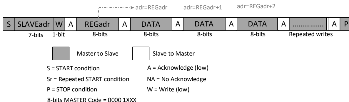
Figure 13: Consecutive Write Command
