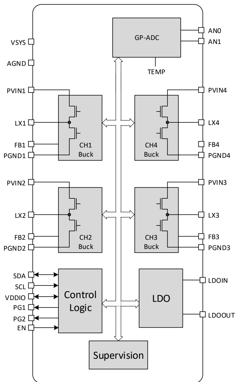
Figure 2: Block Diagram
