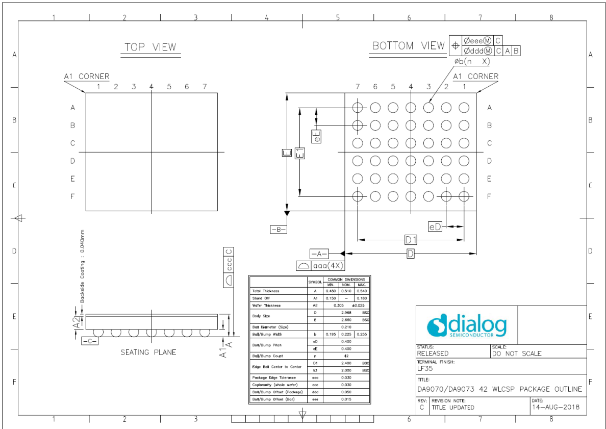
Figure 44: WLCSP-42 Package Outline Drawing, V3 Version
