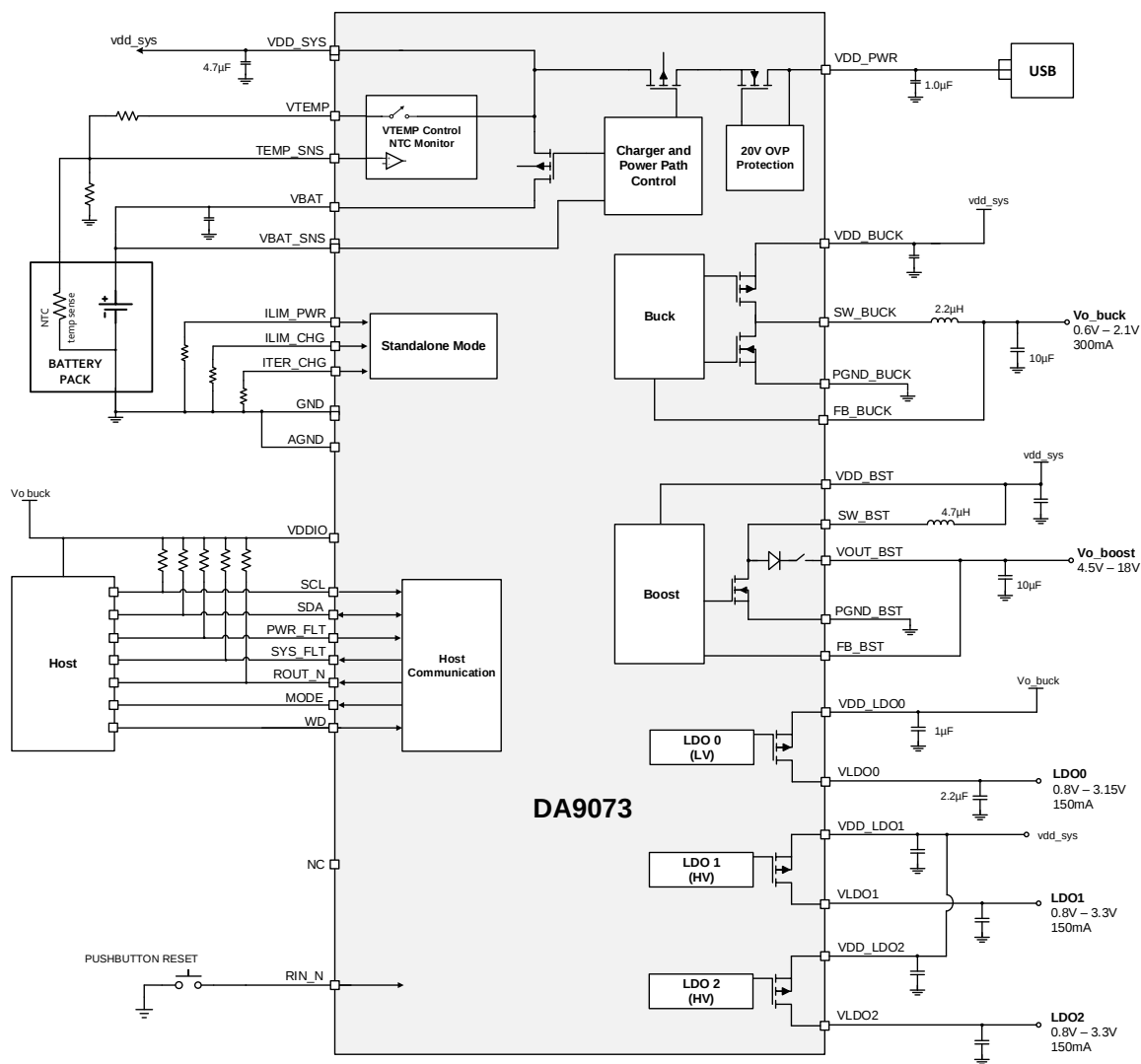
Figure 1: System Diagram
