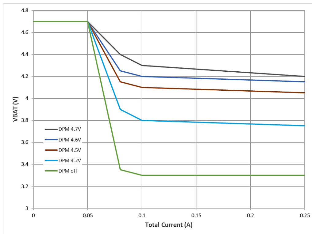
Figure 32: VDD_PWR DPM Setting Recommendations
