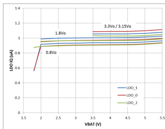
Figure 26: V_{DD\_LDO} IQ, no Load
