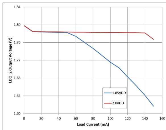
Figure 21: LDO_2 Regulation and Dropout, V_{OUT} = 1.80\text{ V}
