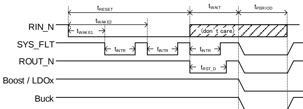
Figure 33: Power-Cycle by Pushbutton Timer
