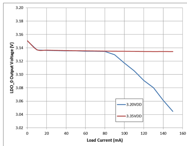
Figure 17: LDO_0 Regulation and Dropout, V_{OUT} = 3.15 \text{ V}
