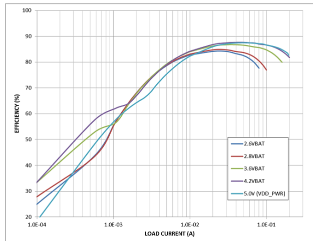
Figure 9: Boost Efficiency, V_{OUT} = 12\text{ V} , V_{IN} = V_{BAT}
