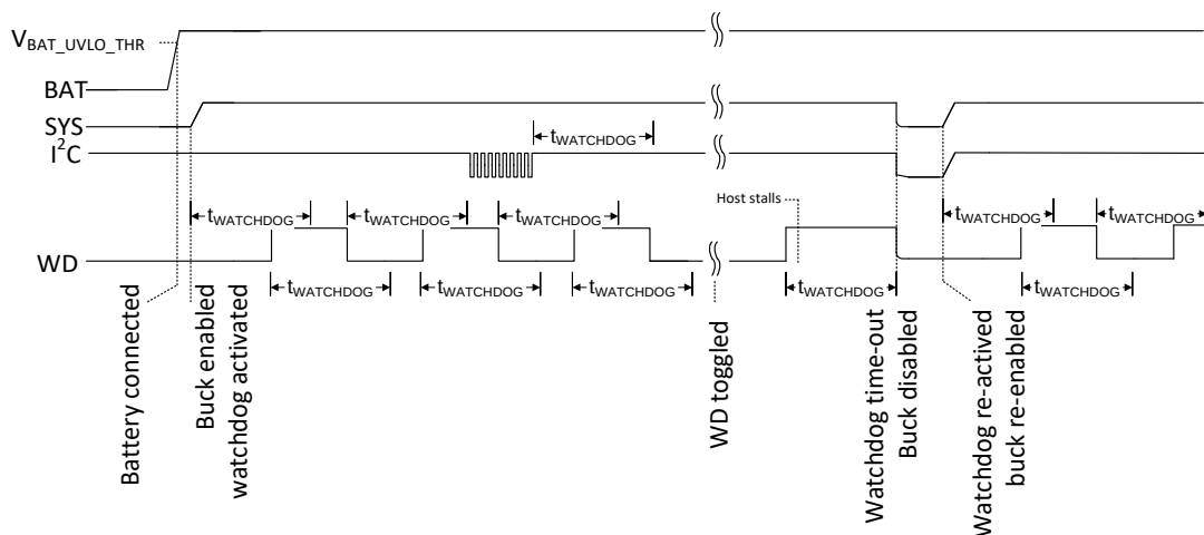
Figure 36: Watchdog Behavior
