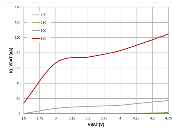
Figure 25: V_{BAT} IQ, Ship Mode
