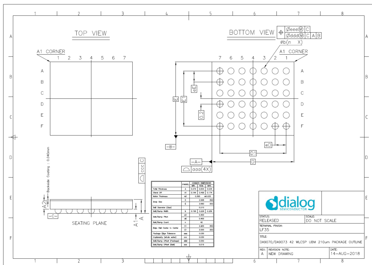
Figure 45: WLCSP-42 Package Outline Drawing, OH Version
