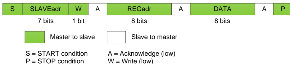
Figure 25: 2-WIRE Byte Write (SI/DATA Line)
