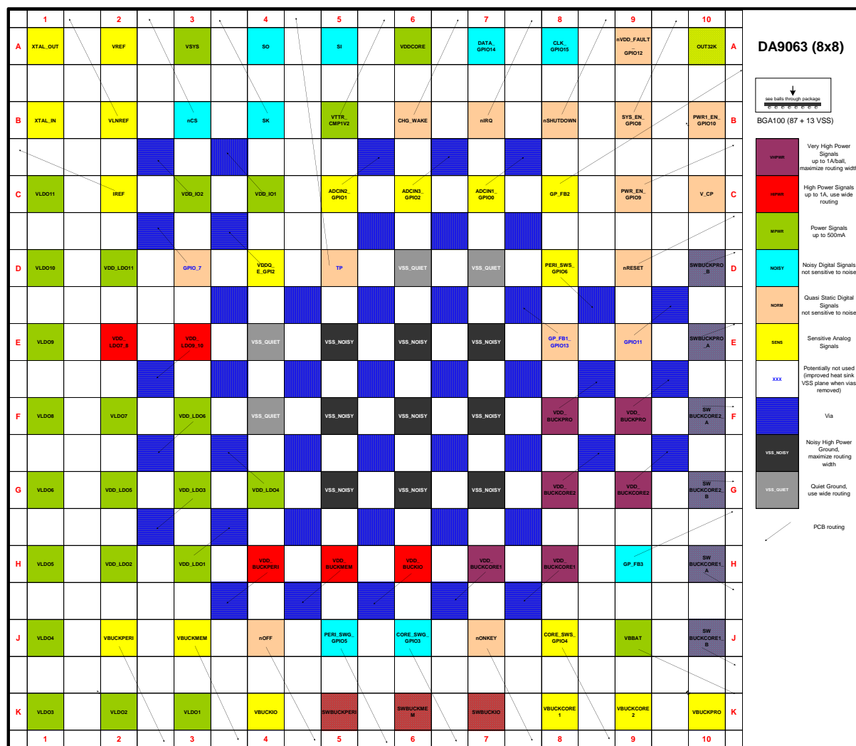
Figure 2: Connection Diagram
