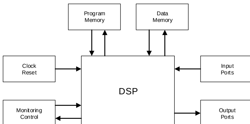
Figure 17. DSP connections
