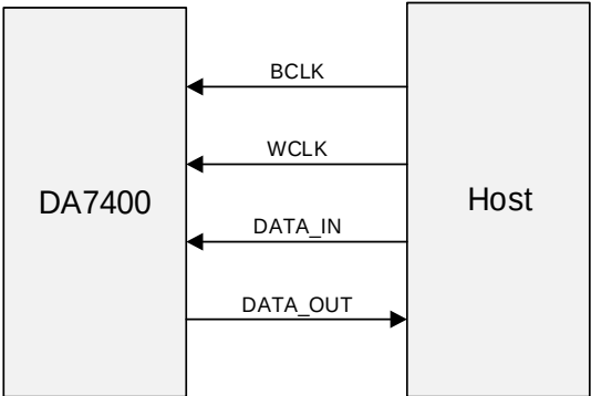
Figure 24. Slave mode
