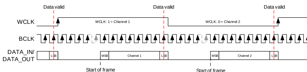
Figure 28. Right-justified format
