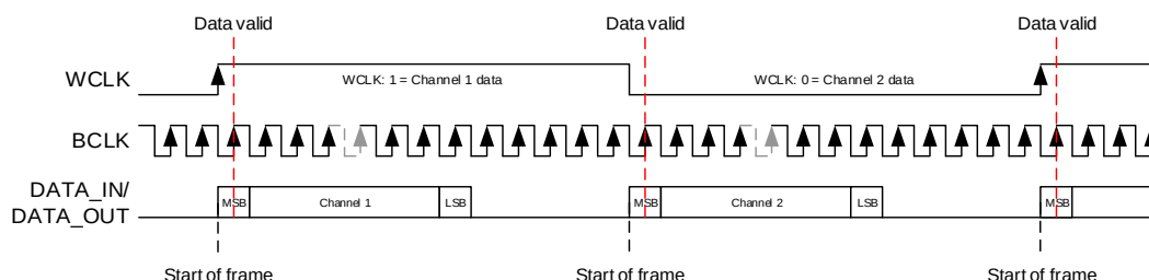
Figure 27. Left-justified format
