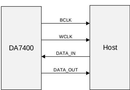
Figure 23. Master mode
