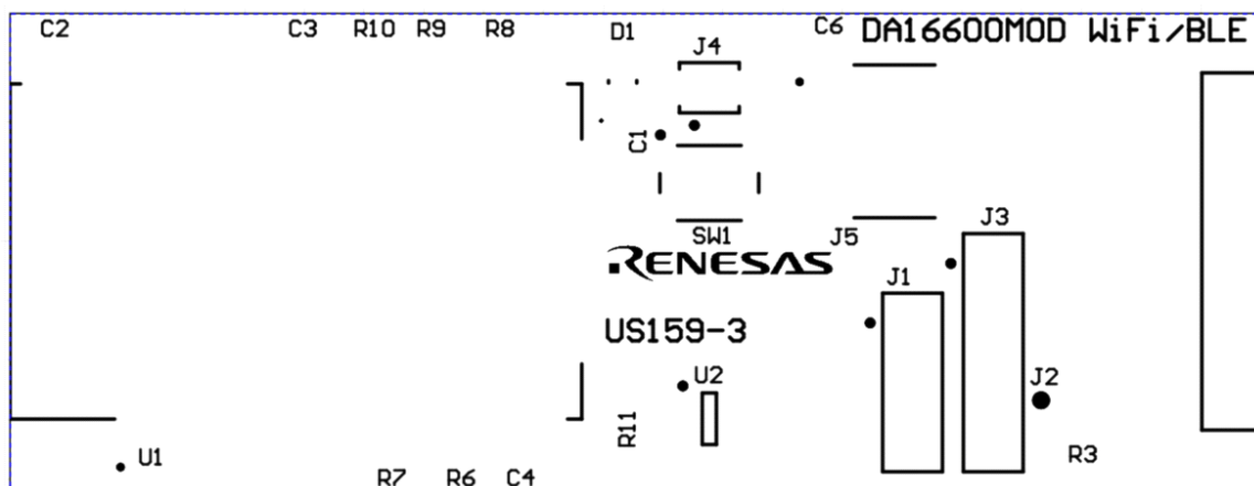
Figure 4. Silkscreen Top
