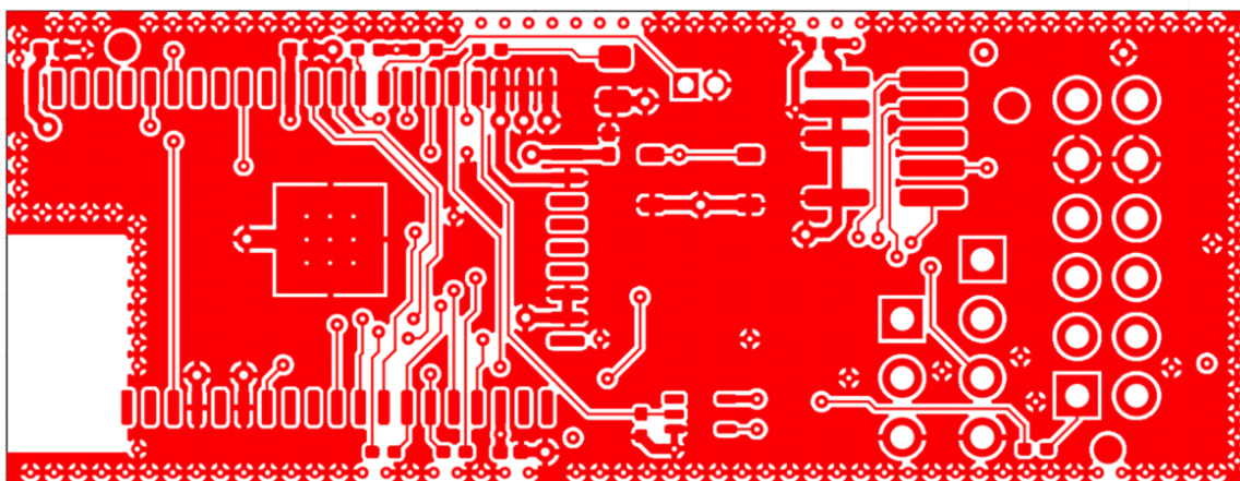
Figure 5. Copper Top
