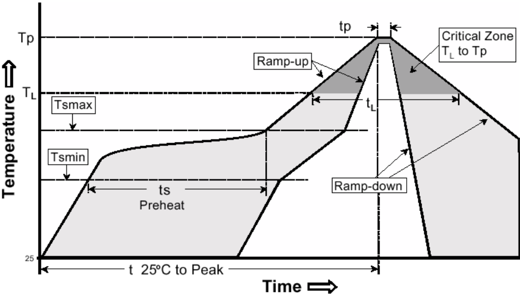
Figure 75: Reflow Condition
