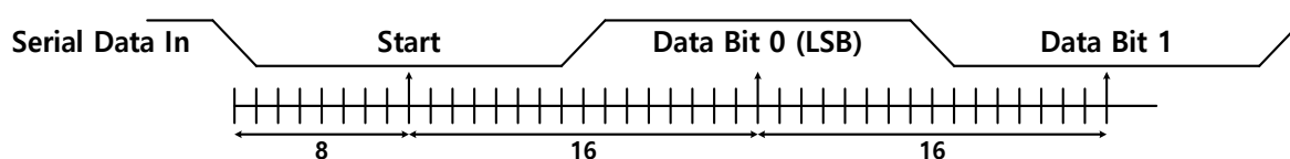
Figure 51: Receiver Serial Data Sampling Points
