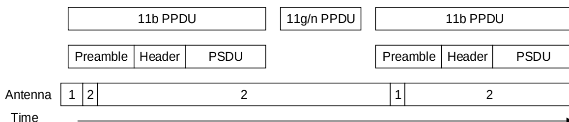
Figure 48: Antenna Switching Timing Diagram
