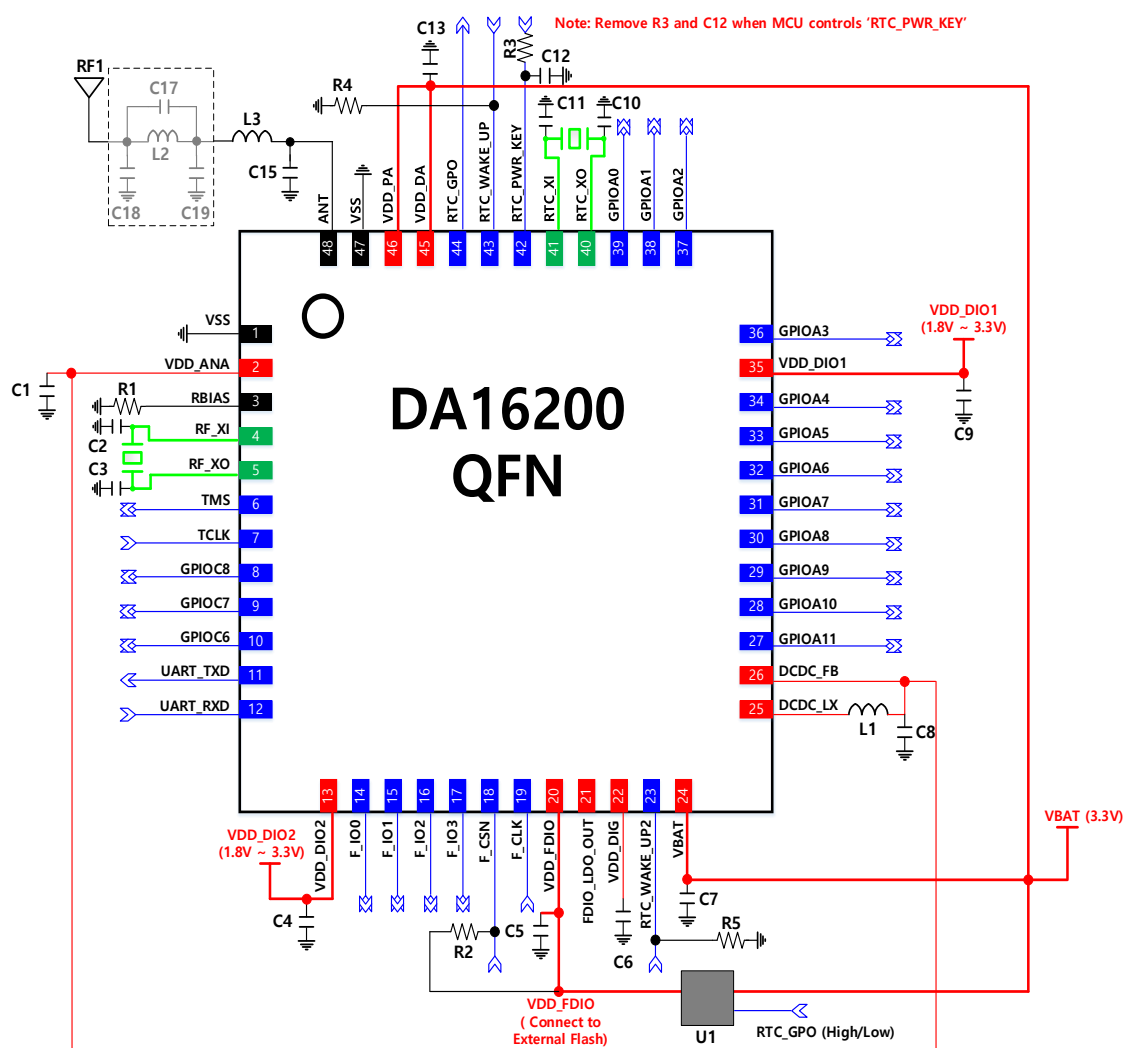
The power supply of the External Flash memory is the same as VDD_FDIO. VDD_DIO1/2 can be connected to the same power source as the external component that is connected to the DA16200. Remove R3 and C12 when an MCU controls 'RTC_PWR_KEY'. Table 375 lists the components for an application that uses the DA16200 OFN in 3.3 V Flash mode.
