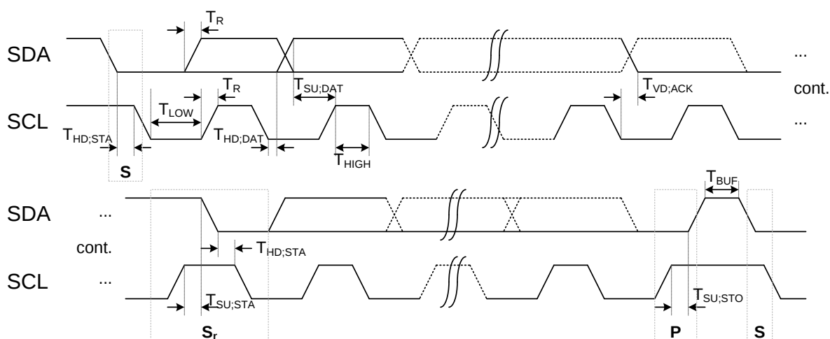
Figure 34: I2C Slave Timing Diagram
