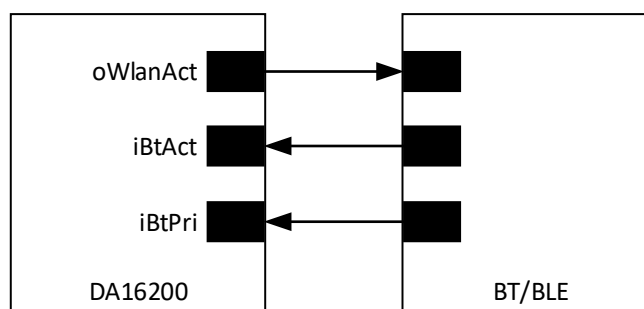
Figure 57: Bluetooth Coexistence Interface
