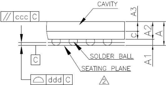
Figure 70: Side View
