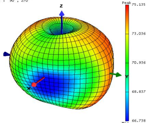
Figure 3: TIS 3D
