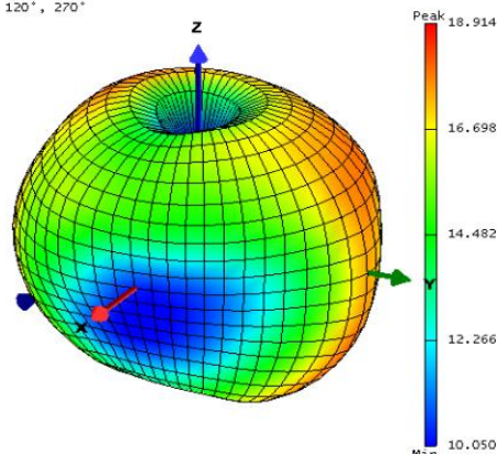
Figure 4: TRP 3D
