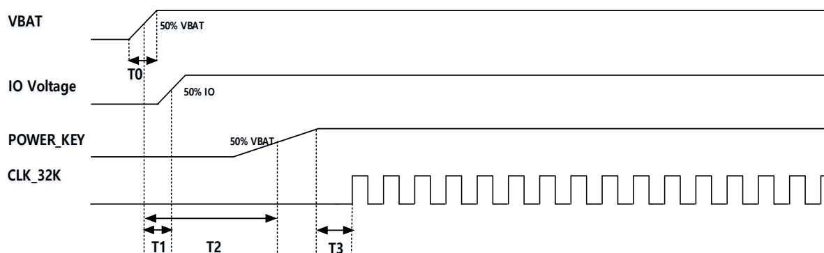
Figure 5: Power-on Sequence
