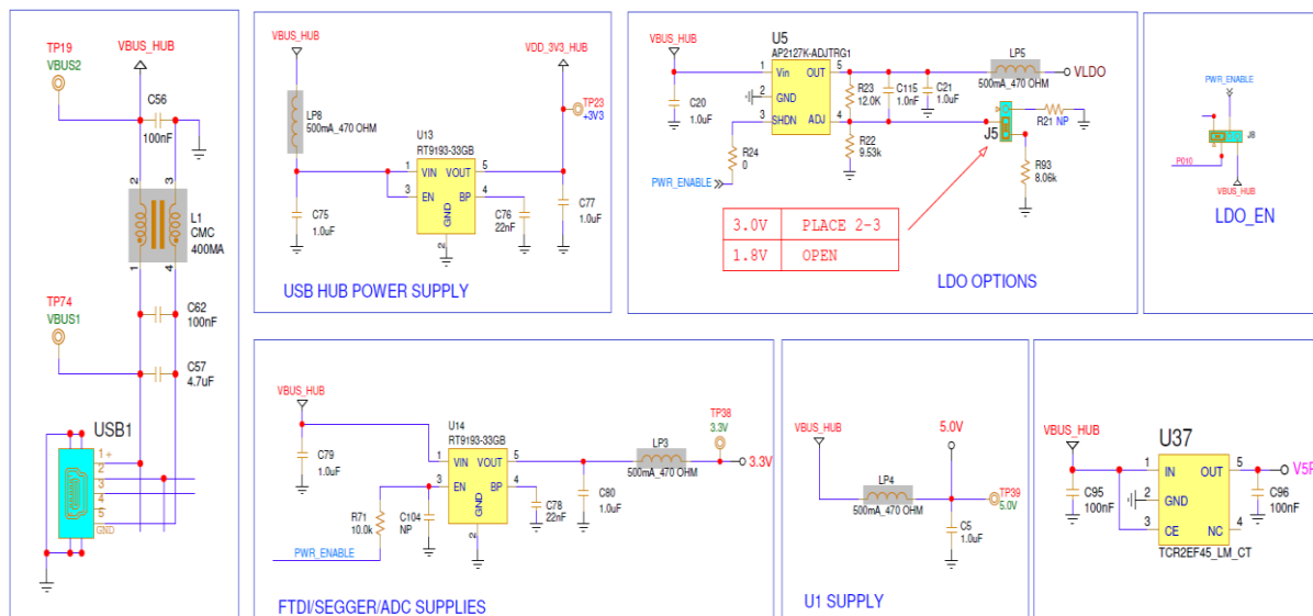
Figure 28. DA1459x Pro-Motherboard Power section
