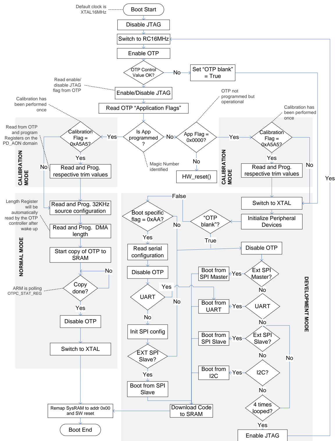
Figure 12: BootROM Sequence
