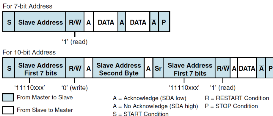
Figure 35: Master-Receiver Protocol
