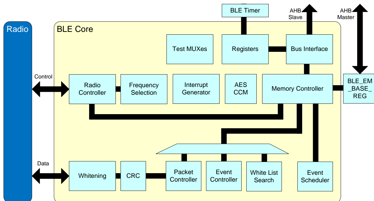
Figure 78: Bluetooth® LE Core Block Diagram
