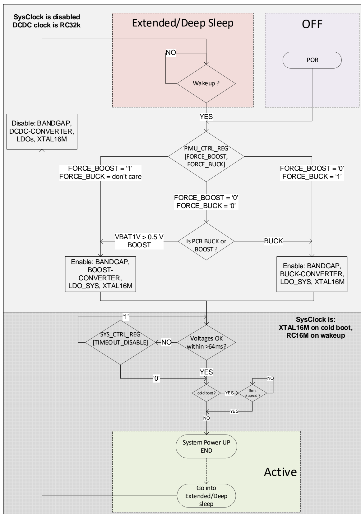
Figure 10: Power/Wake-Up Sequence
