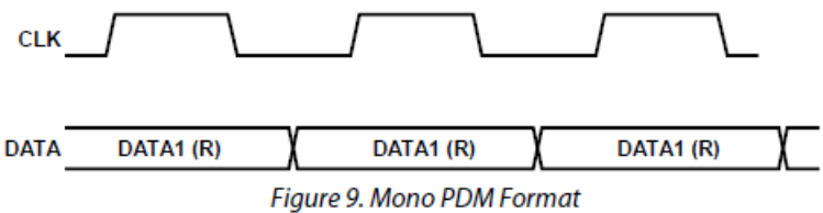
Figure 9. Mono PDM Format
