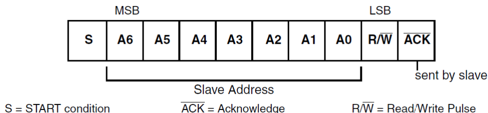
Figure 32: 7-bit Address Format
