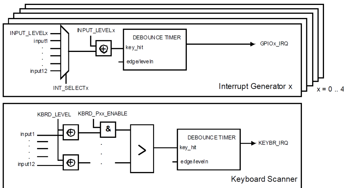
Figure 65: Keyboard Controller Block Diagram
