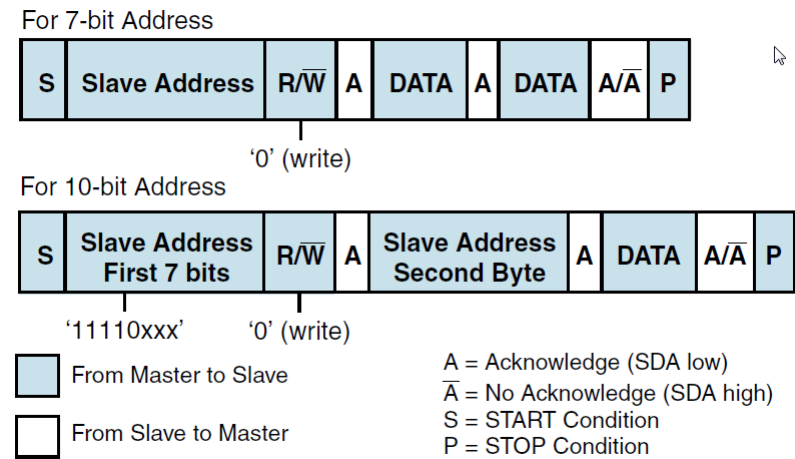
Figure 39: Master-Transmitter Protocol
