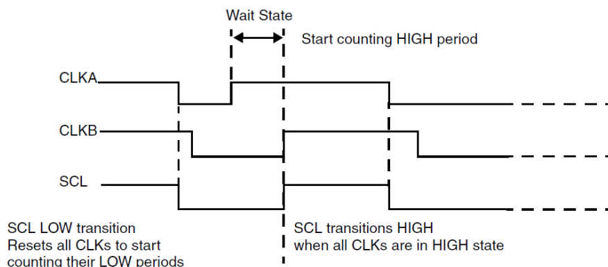
Figure 43: Multiple Master Clock Synchronization
