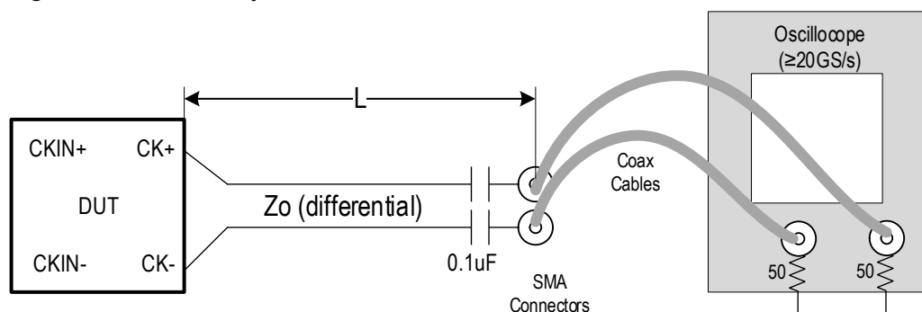
Figure 6. Test Setup for PCIe Clock Phase Jitter Measurements
