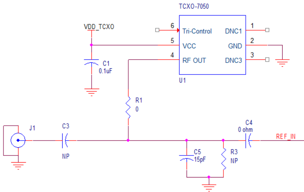
Figure 3. Input Schematic
