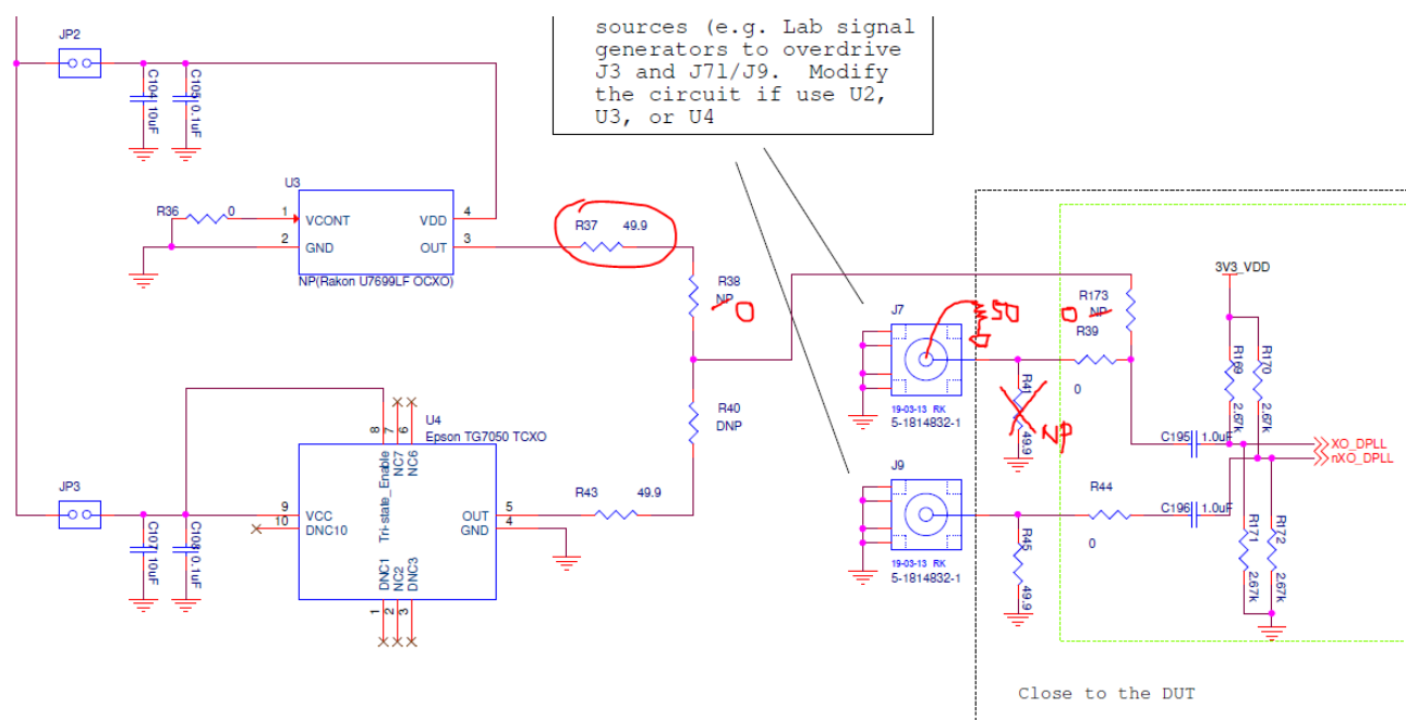
Figure 16. Use On-board OCXO to Drive the XO Input
