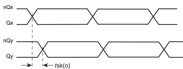
Figure 6. Output Skew
