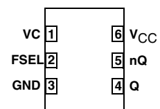
IDT8N4DV85 6-lead ceramic 5mm x 7mm x 1.5mm package body CD Package Top View
