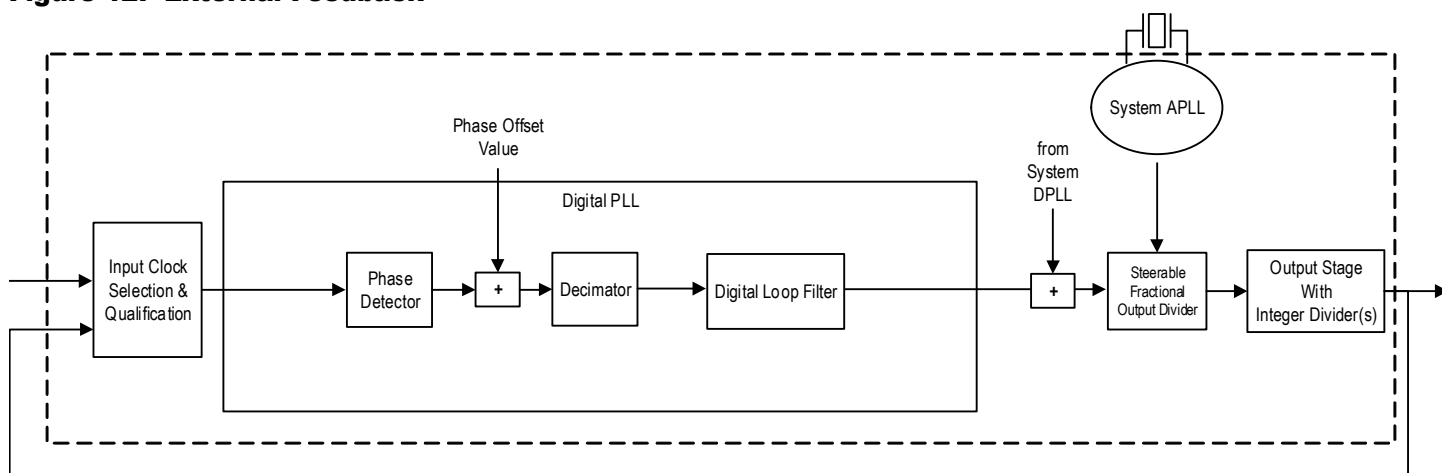
Figure 12. External Feedback
