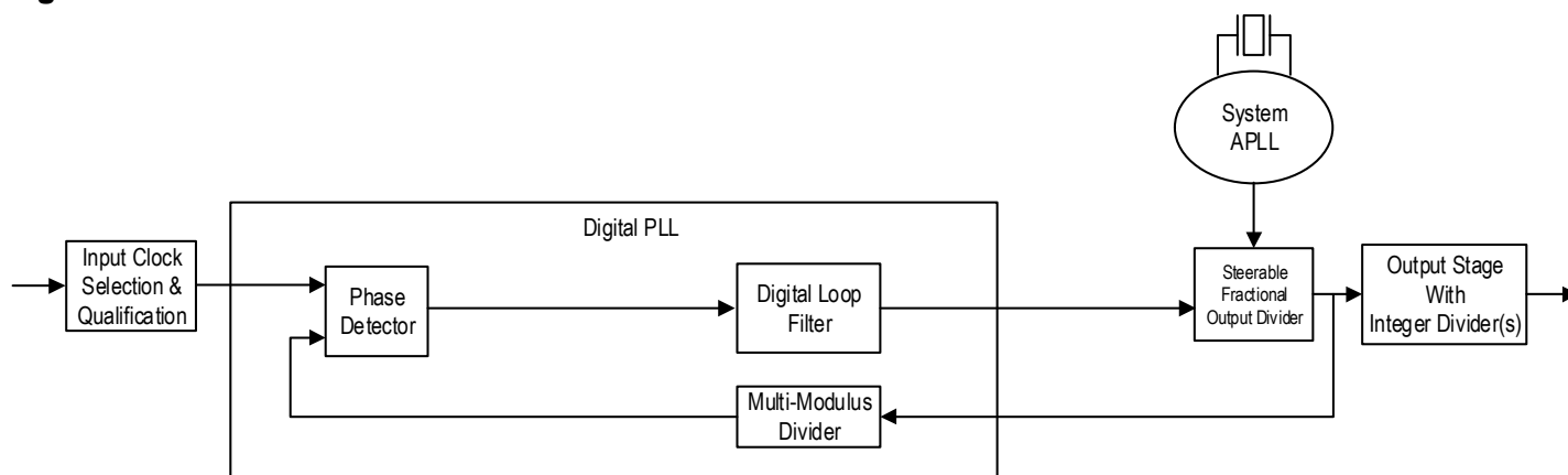
Figure 10. DPLL Channel
