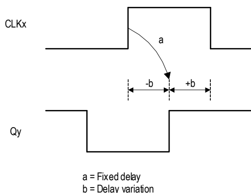
Figure 40. Input-Output Delay with Internal Feedback
