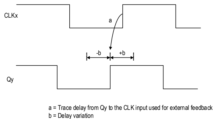
Figure 47. Input-Output Delay with External Feedback
