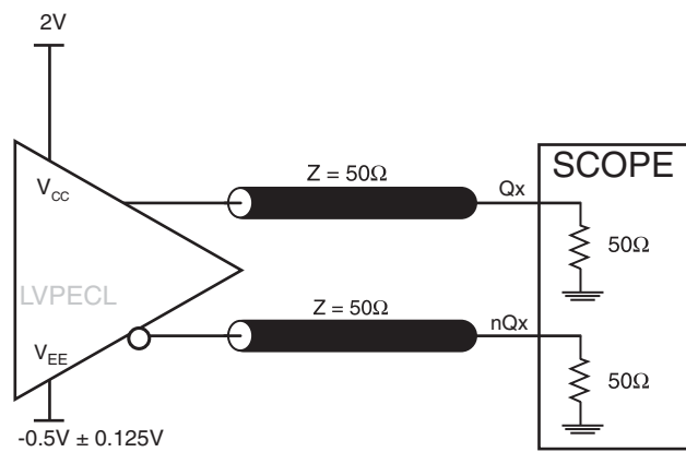
OUTPUT LOAD 2.5V AC TEST CIRCUIT
