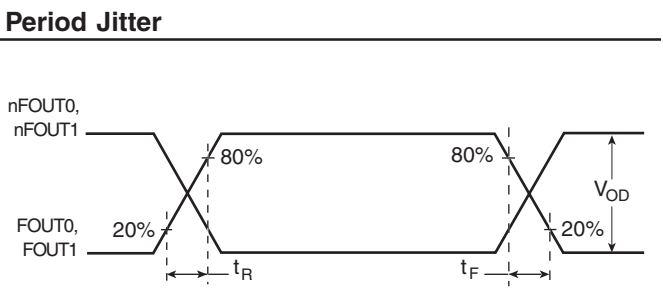
OUTPUT RISE/FALL TIME
